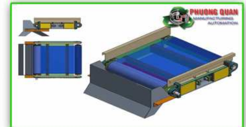
Magnetic roller conveyor
